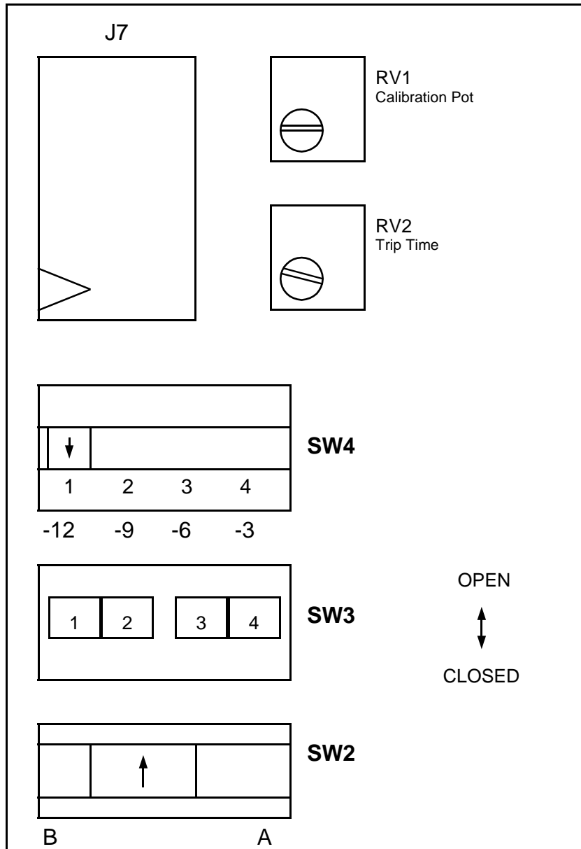
Figure 5.2 CALIBRATION ADJUSTMENTS
