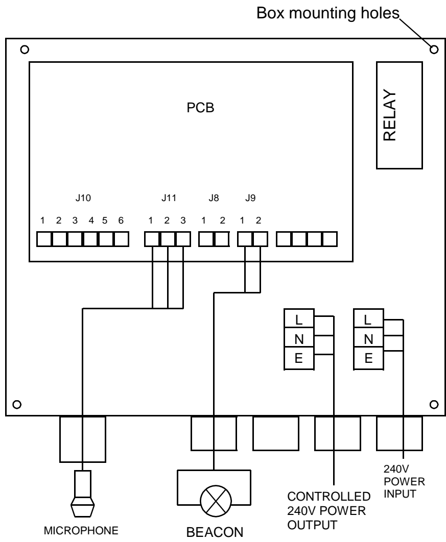
Figure 3.1 WIRING SCHEMATIC
